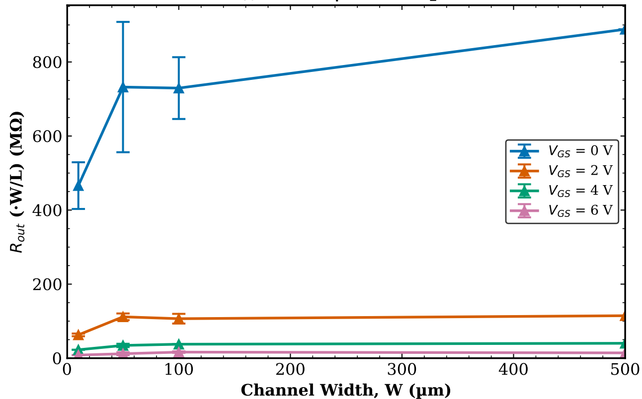
TFT1 Combined (Tr. 1 & 2) R_{out} vs W | L = 40\text{ }\mu\text{m}
